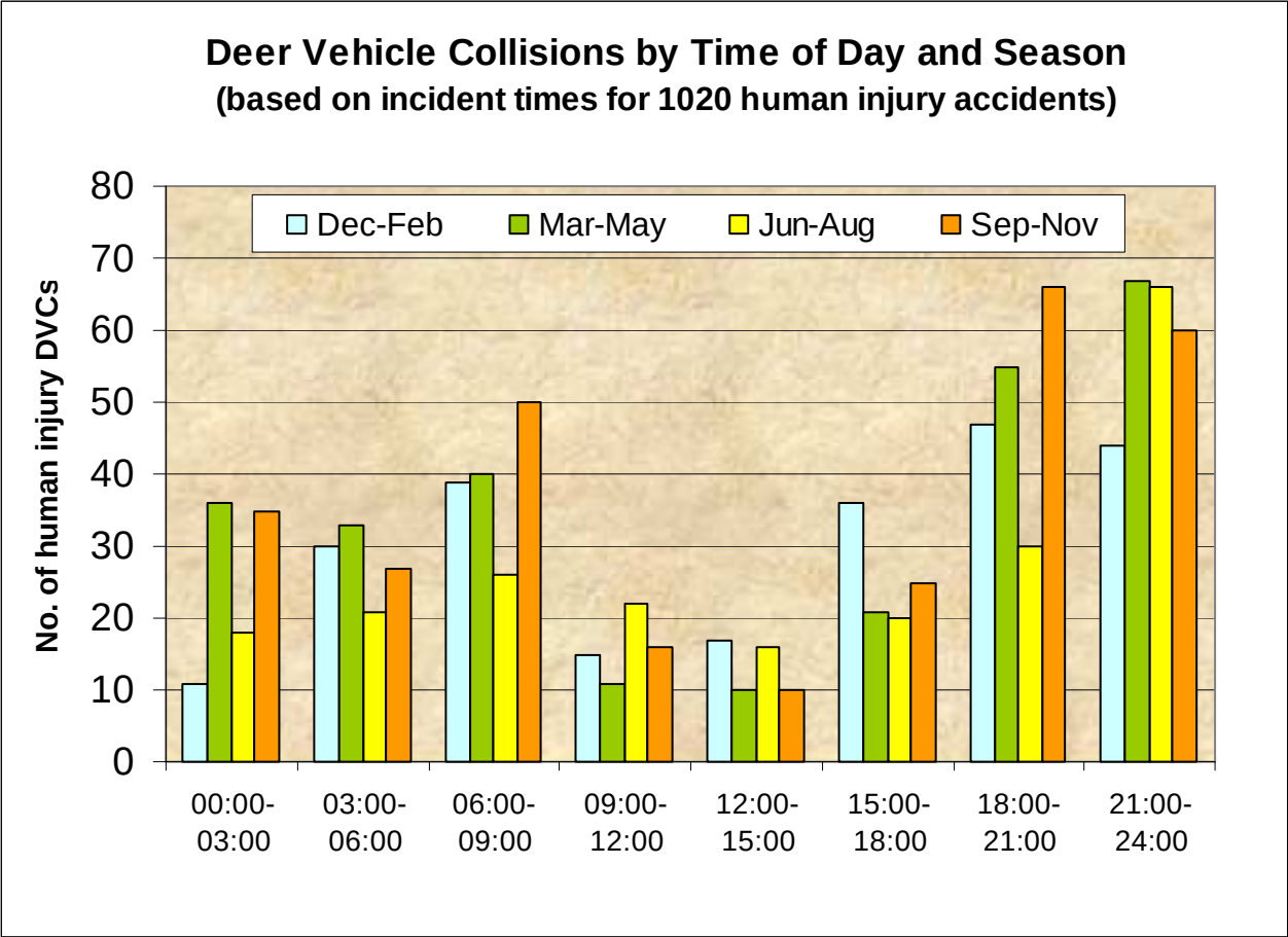
Figure 3: Daily accident peaks and the influence of season. (analysis is restricted to human injury accidents only, as incidents times tend to be recorded most accurately and reliably for that sub-set of data)
